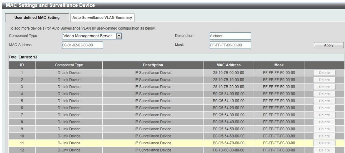
Figure 7-17 User -defined MAC Settings window
