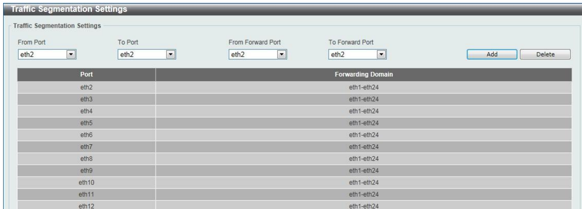
Figure 9-2 Traffic Segmentation Settings window
